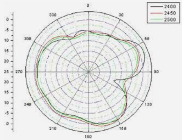
2.4G (PHI=90)
