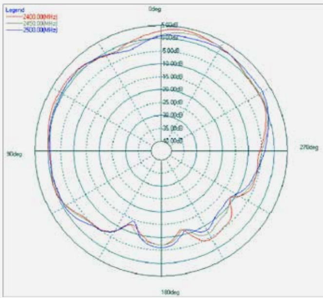
2.4G (PHI=0)
