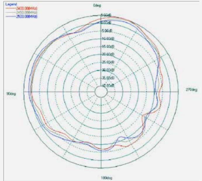
2.4G (PHI=90)
